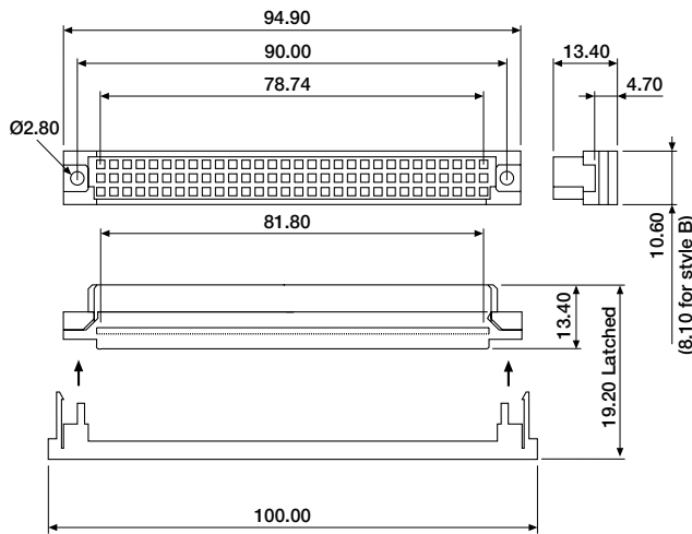
Drawing is representative of style C.
