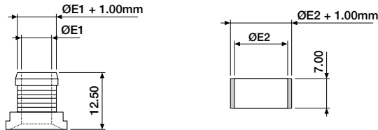
outer ferrule
