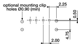
Header right angle, single row
