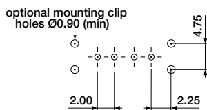
Header straight, single row
