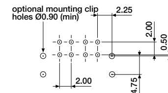
Header right angle, double row
