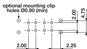
Header straight, double row
