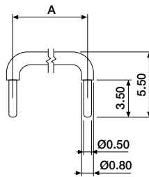
USP-1000-1500 A = 2.54 tin plated USP-1000-1520 A = 2.54 gold plated USP-2000-1500 A = 5.08 tin plated USP-2000-1520 A = 5.08 gold plated
