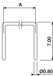
USP-1000-0820 A = 2.54 gold plated USP-2000-0820 A = 5.08 gold plated
