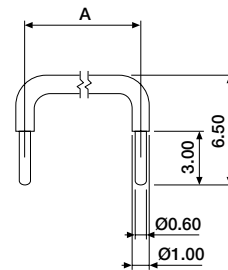
USP-1000-1600 A = 2.54 tin plated USP-1000-1620 A = 2.54 gold plated USP-2000-1600 A = 5.08 tin plated USP-2000-1620 A = 5.08 gold plated USP-3000-1600 A = 7.62 tin plated USP-3000-1620 A = 7.62 gold plated USP-4000-1600 A = 10.16 tin plated USP-4000-1620 A = 10.16 gold plated
