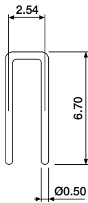
USP-1000-0520 gold plated
