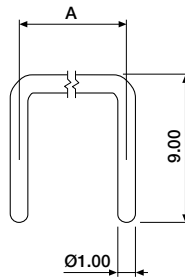
USP-2000-1100 A = 5.08 tin plated USP-2000-1120 A = 5.08 gold plated USP-4000-1100 A = 10.16 tin plated USP-4000-1120 A = 10.16 gold plated
