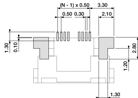
FUZ-XXSM-3640 (30 to 50 circuits)
