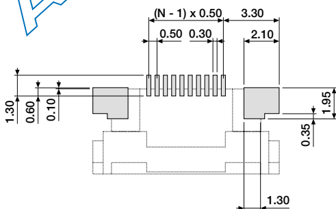
FUZ-XXSM-3640 (05 to 30 circuits)
